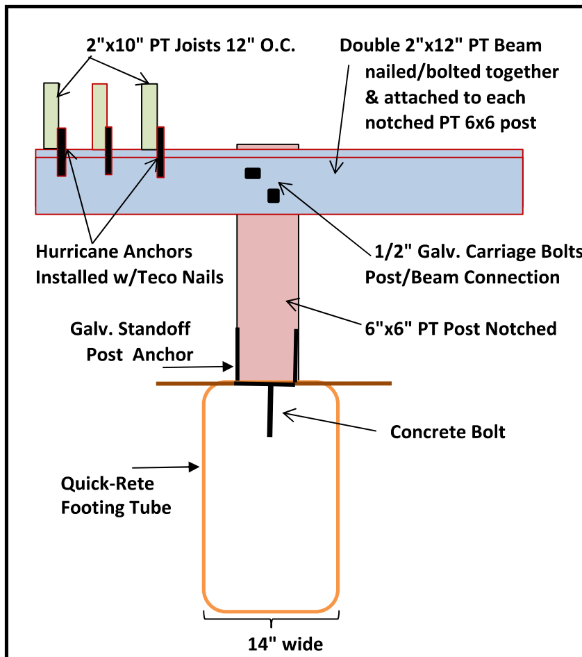
DIAGRAM FOR DECK STRUCTURE
