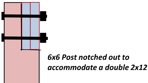
SIDE VIEW POST TO BEAM CONNECTION
