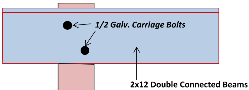
DIAGRAM POST TO BEAM CONNECTION
