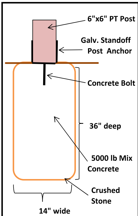
DIAGRAM FOR DECK FOOTING
