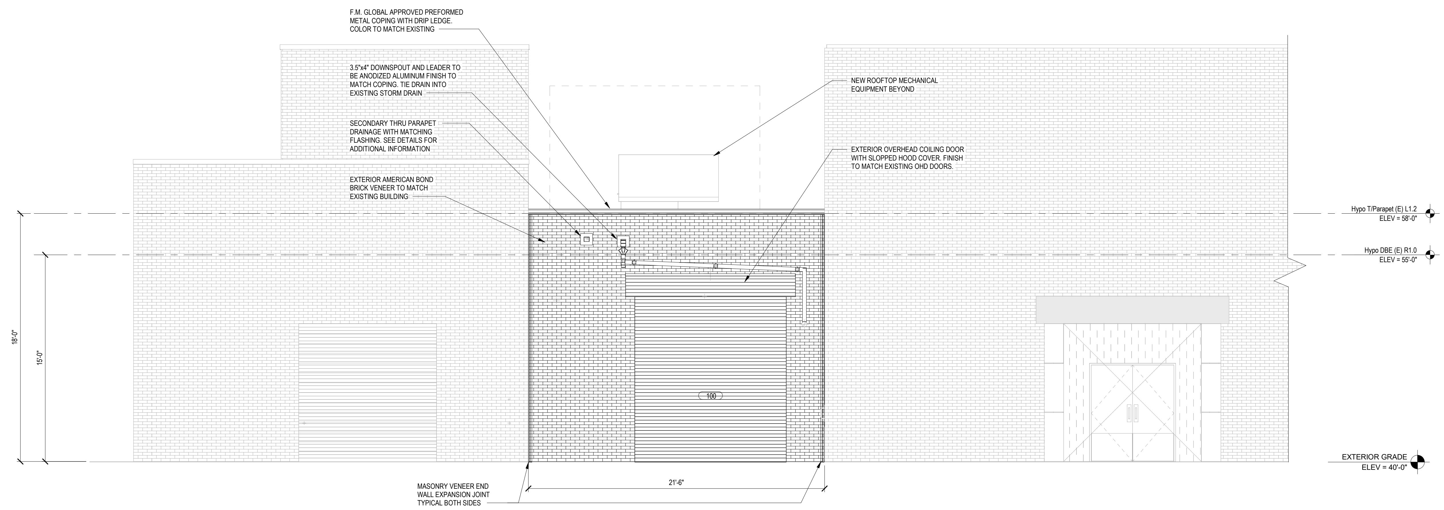
1 ELEVATION - NORTH SCALE: 1/4" = 1'-0"
