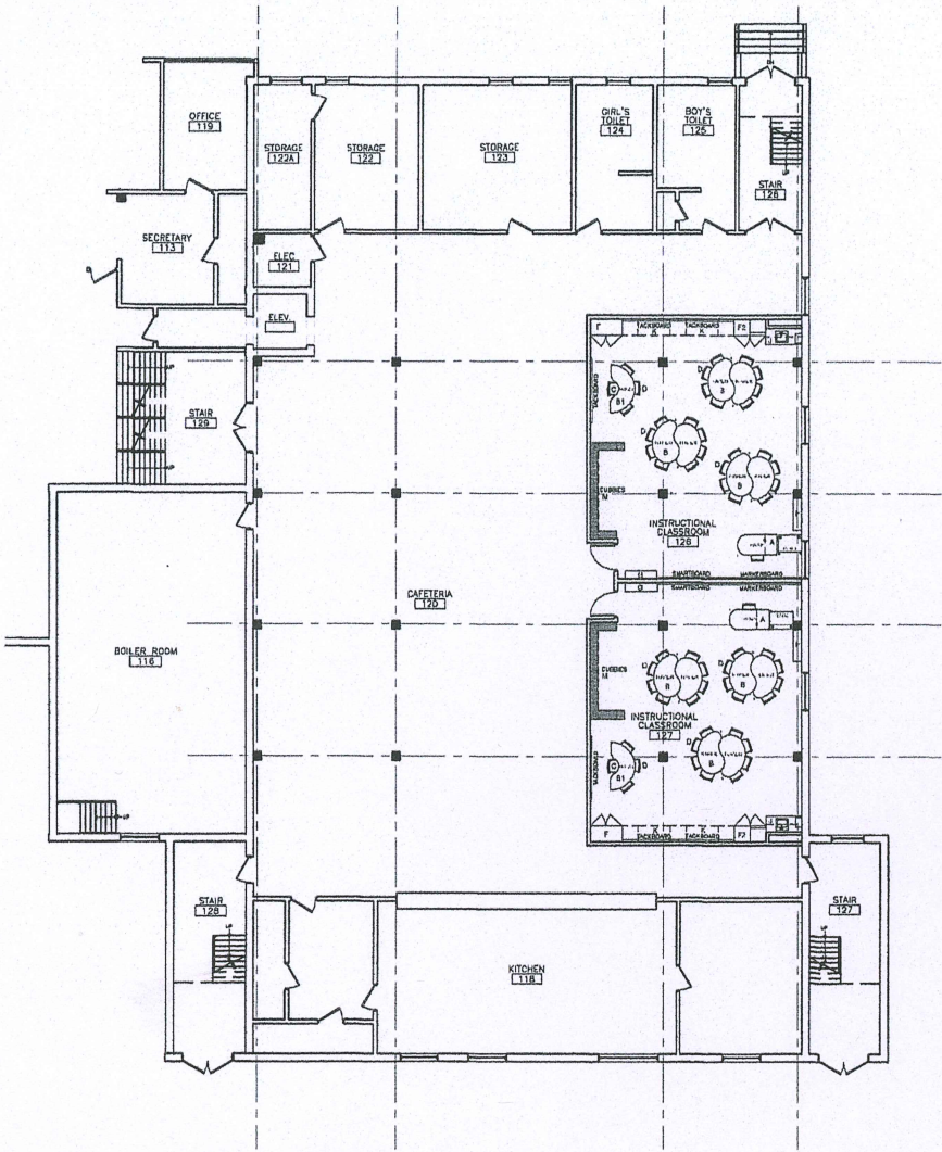
1 FIRST FLOOR PLAN A-101 SCALE: 1/8"=1'-0" LOCATION: FIRST FLOOR
