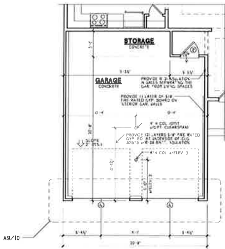
02 GARAGE w/SLAB OPTION SCALE: 1/4"=1'-0"
