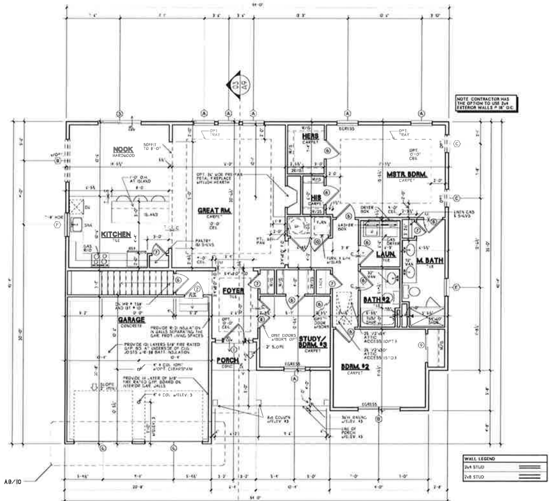
01 FLOOR PLAN - ELEV. 01 & 02 SCALE: 1/4"=1'-0"
