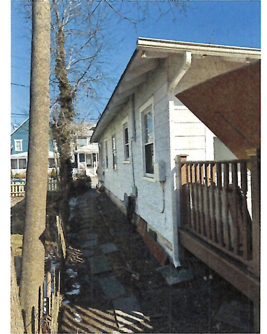
EXIST'G LEFT SIDE VIEW FACING STREET
