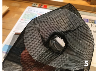
5. A section of the screening should overlap to keep the insects from escaping. 6. If you are using flexible screening that can't support itself, use hot glue to attach the screening to the plastic top.
