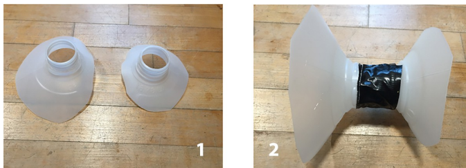
1. Cut the tops from two plastic milk jugs. 2. Attach them together with hot glue and/or duct tape.
